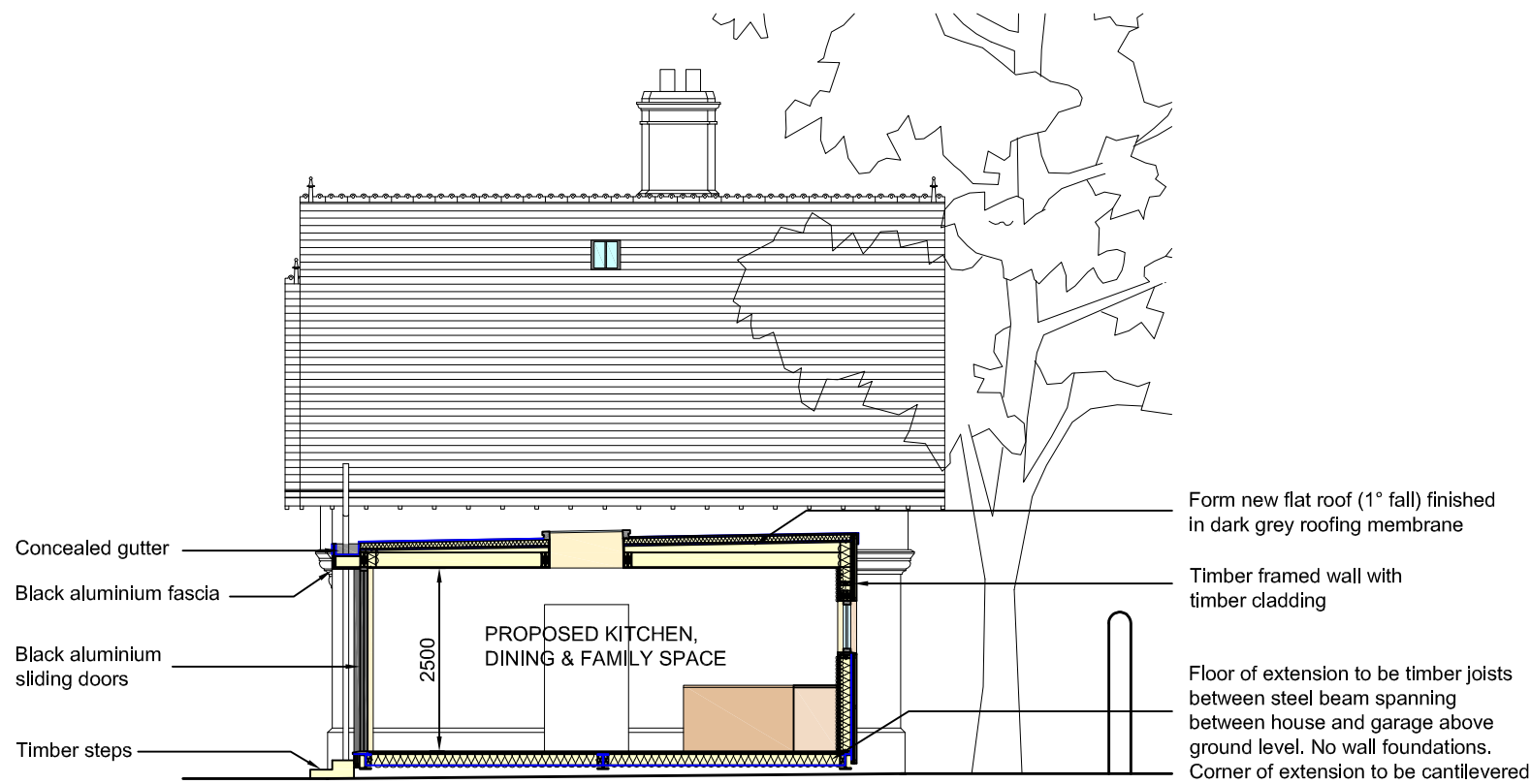
PROPOSED SECTIONAA 1:100
